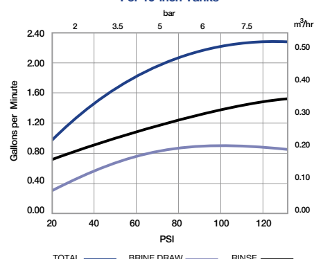
Injector "N" (Green) For 16-inch Tanks
