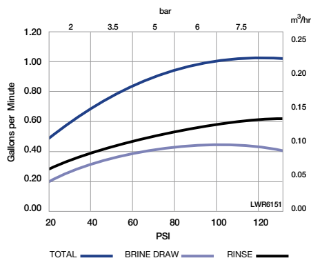
Injector "K" (Pink) For 12-inch Tanks
