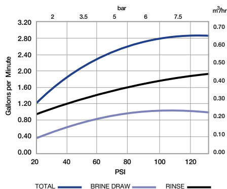
Injector "Q" (Purple) For 18-inch Tanks
