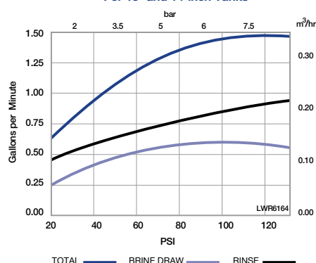
Injector "L" (Orange) For 13- and 14-inch Tanks
