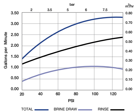
Injector "R" (Dark Grey) For 21-inch Tanks
