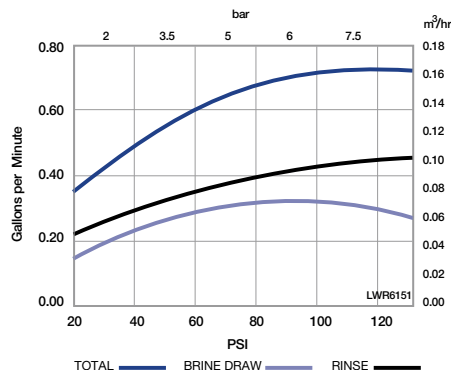
Injector "J" (Light Blue) For 10-inch Tanks
