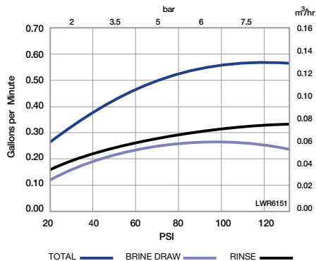
Injector "H" (Light Purple) For 9-inch Tanks
